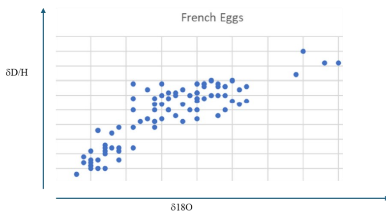
Fig. 1. The figure above gathered all isotopic results. Each sample is represented by its isotopic couple (Delta ^{18}O , D/H).
