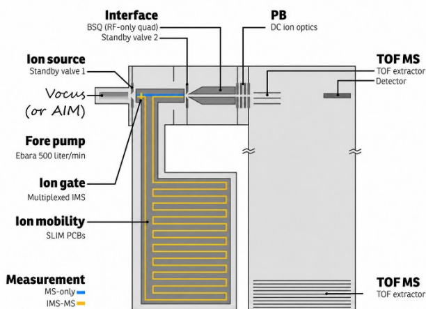
Fig. 1. Schematic representation of the Vocus HR-CI-IMS-TOF instrument
