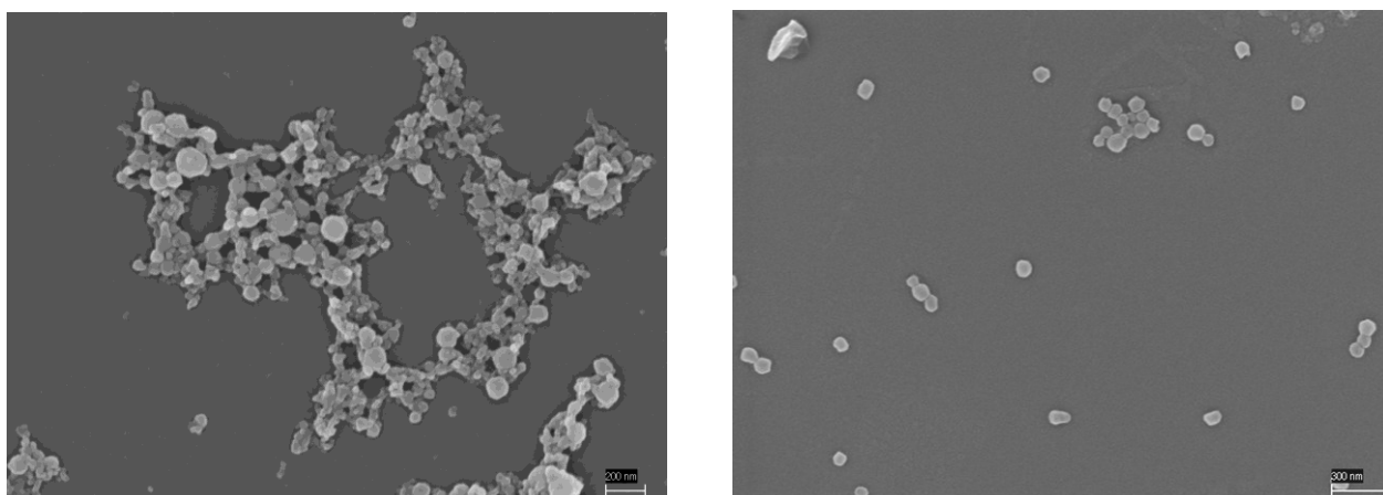
Fig. 1. SEM images of unloaded (A) and peptides-loaded (B) zein-based nanoparticles.
