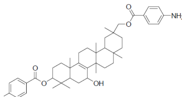
Fig. 2. Multiflorane-type triterpenoid
