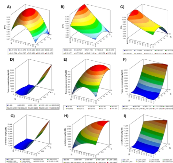
Figure 1. Response surface plots showing the effect of extraction parameters on extraction yield (A, B, C), trans-resveratrol (D, E, F) and \epsilon -viniferin (G, H, I). Plots report the data correlation of S vs. t (A, D, G), R vs. t (B, E, H), and R vs. S (C, F, I).
