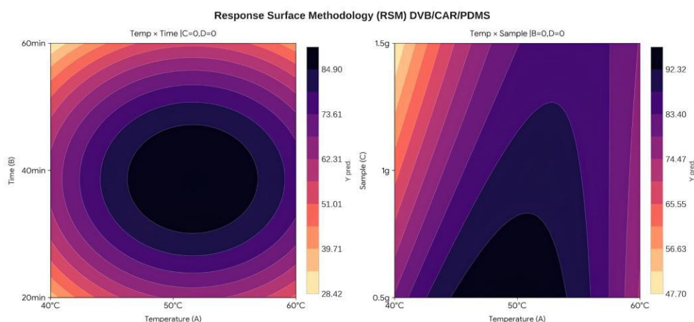
Fig. 1. Response surface plots illustrating the interactive effects of extraction temperature (°C), extraction time (min), and sample amount (g) on the total area of VOCs.
