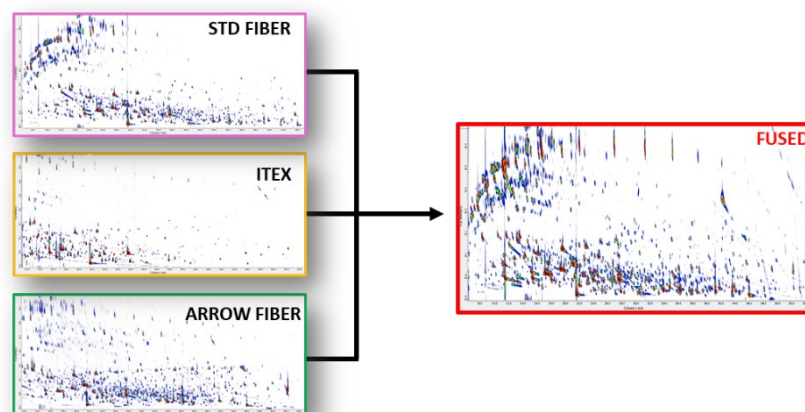
Figure 1. Chromatographic data fusion of complementary headspace extraction techniques. Individual GC×GC chromatograms acquired using SPME fiber, SPME Arrow and ITEX were combined to generate a single fused chromatogram for unified downstream data processing and interpretation.
